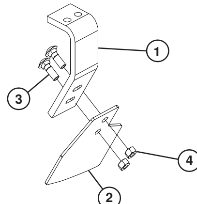
SCRAPER BLADE ASSY LH OFFSET (SHOWN) SCRAPER BLADE ASSY RH OFFSET
